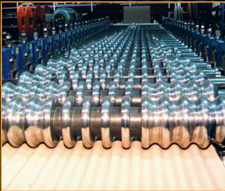
The IRONCLAD™ Panel Rollformer
